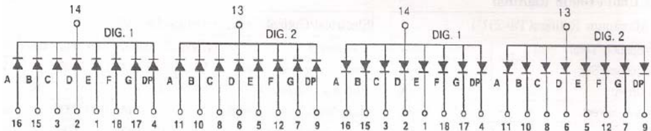
Cathode Common(MD-620)
